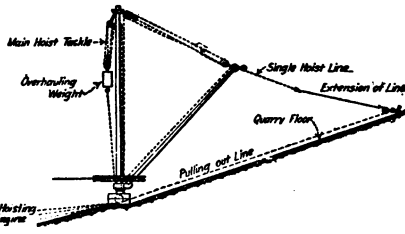
Fig. 133B. Removing Granite Blocks.
